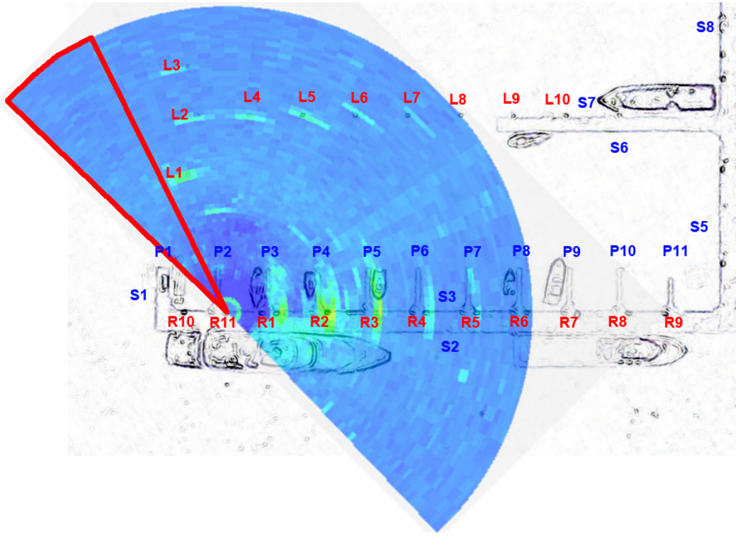
Fig. 2: Overlay of median statistics of the scanline measurements image with satellite view of potential targets at RSYC. A background sector to the portside of the sonar can identified by the red triangle.
