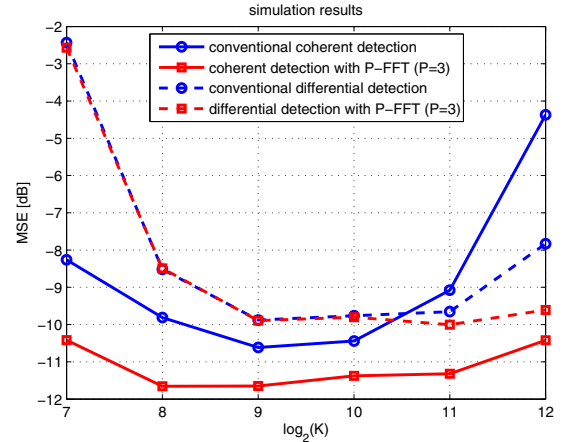
Fig. 7. Average MSE performance obtained via simulation. The simulated channel parameters are selected to match those of the experimental channel, observed for the experimental data as described in Sec. III-A, and similar receiver configurations are used. The MSE results demonstrate the same trend as those observed for the experimental data.
