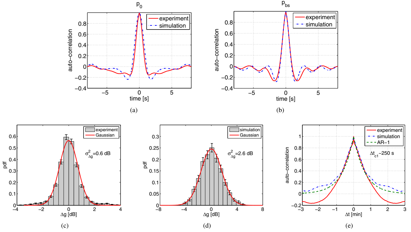
Fig. 5. Small-scale (top) and large-scale (bottom) statistics of the experimental and the simulated channels: time-correlation functions corresponding to (a) the direct path, and (b) the bottom-surface path; histogram of (c) experimental and (d) simulated gain and Gaussian approximation; (e) time-correlation of experimental and simulated gain and AR-1 auto-correlation.
