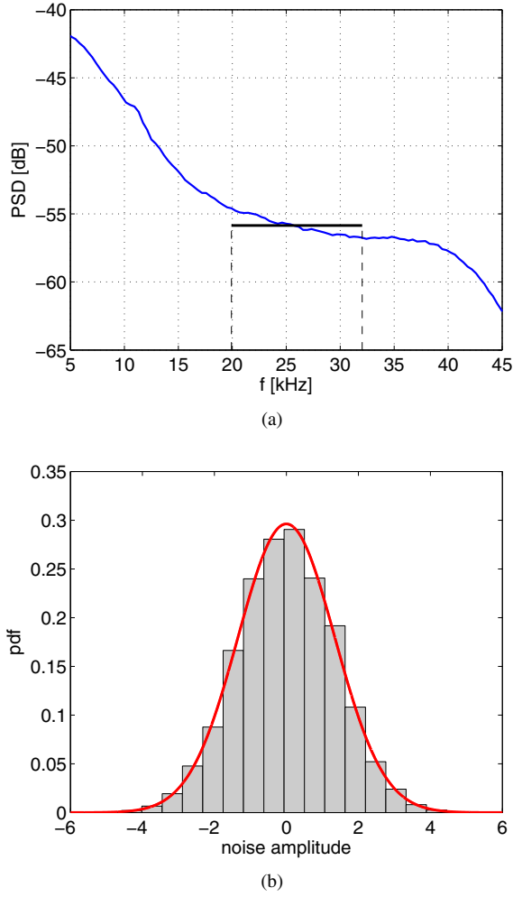
Fig. 8. Noise statistics, estimated from 120 seconds of recording of ambient noise during the experiment: (a) p.s.d., (b) p.d.f. The psd is obtained by the Welch method, using an FFT of size 256 with 50% overlap.
