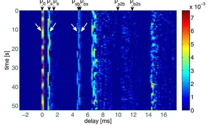
Fig. 4. Time-evolution of the magnitude baseband impulse response of the KAM'11 channel. Specified on top are the nominal path delays.
