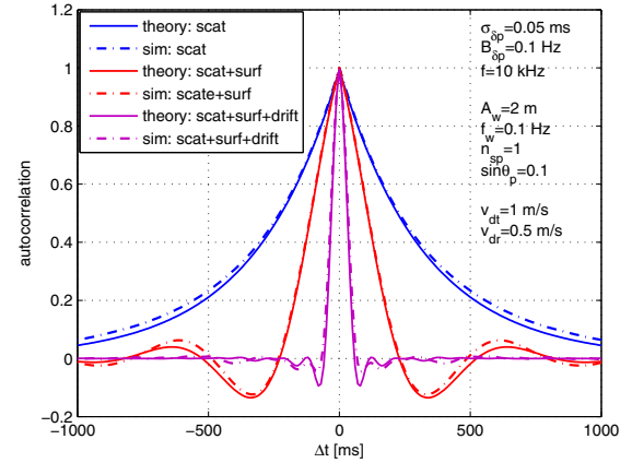
Fig. 2. Time-correlation of the small-scale coefficient \tilde{\gamma}_p in the presence of surface and drifting motion.
