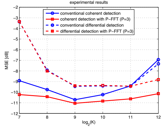
Fig. 6. Average MSE performance for the KAM'11 experiment. The average SNR is observed to be 15 dB at each receiver element within the signal bandwidth. Averaging is performed over 5 \times 10^4 QPSk symbols which were transmitted in 3 frames separated by 3 hours.
