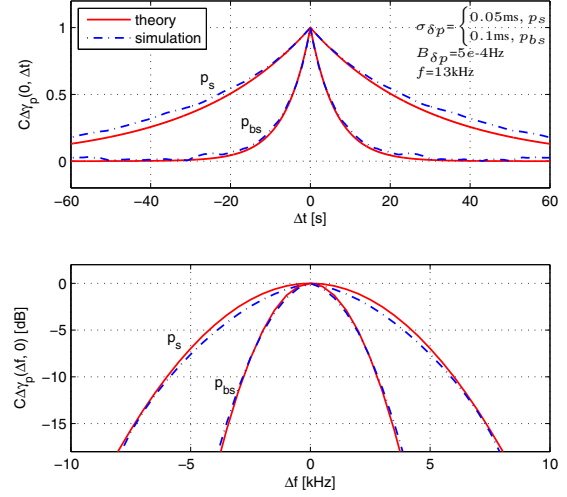
Fig. 1. Time (top) and frequency (bottom) correlation functions, obtained theoretically and via simulation for surface scattered ( p_s ) and bottom-surface ( p_{bs} ) paths.
