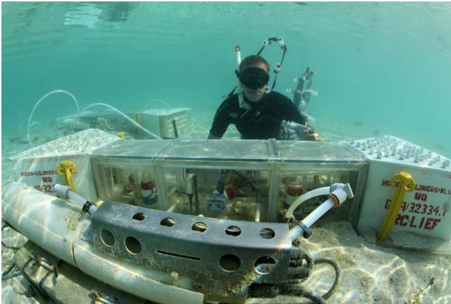
Figure 4: The cpFOCE as deployed at Heron Island
