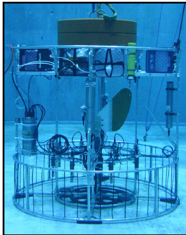
Figure 2: Proto FOCE in the test tank at MBARI Image courtesy of Todd Walsh © MBARI 2005
