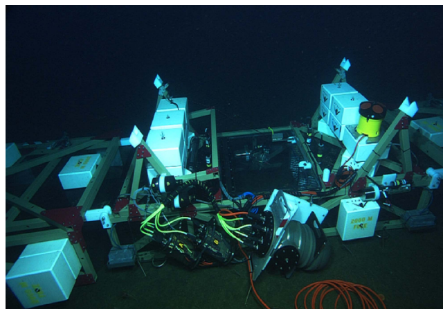
Figure 3: dpFOCE deployed at the Monterey Accelerated Research Site (MARS) in the Monterey Bay
