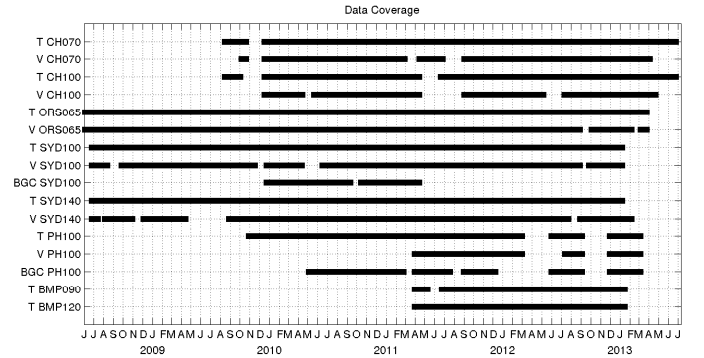
Fig. 2: Data return from the NSW-IMOS mooring array from each of the moorings as identified in Table I and Figure 1. Temperature, velocity and Biogeochemistry sensors are indicated by T, V and BGC respectively.
