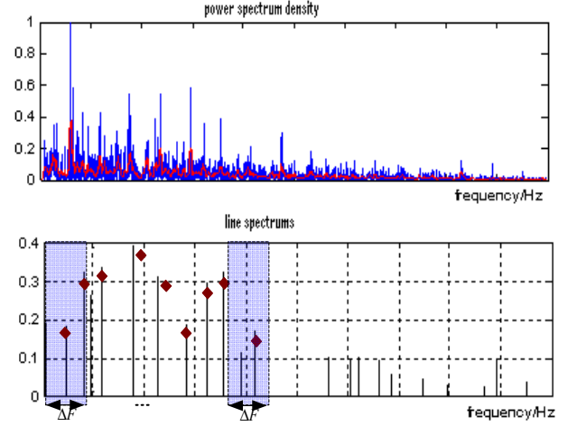
Fig.3 PSD and extracted line spectrums
