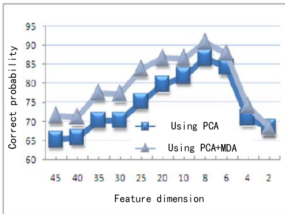
Fig.5 performance comparison(PCA+MDA)
