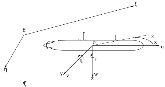
Fig. 6. ITTC coordinate system
