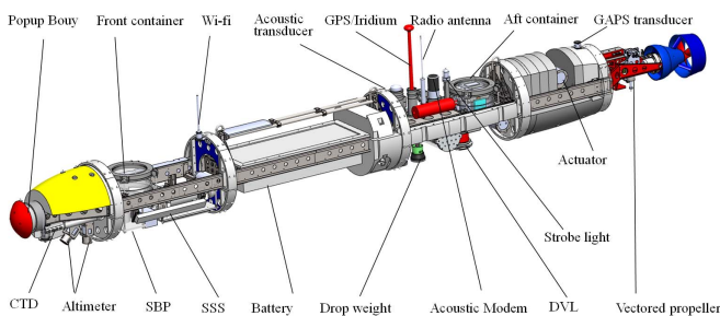
Fig. 2. General internal layout of the seafloor surveying AUV
