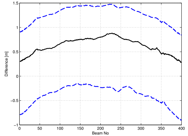
Fig. 1. Mean profile difference between 2.5 minutes of EM710 real-time measurements and a DTM based on post-processed EM1002 measurements (black) as a function of beam number, along with the standard deviation (broken blue).
