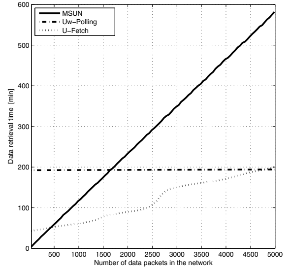
Figure 3. Data retrieval time vs. number of data packets generated in the network.
