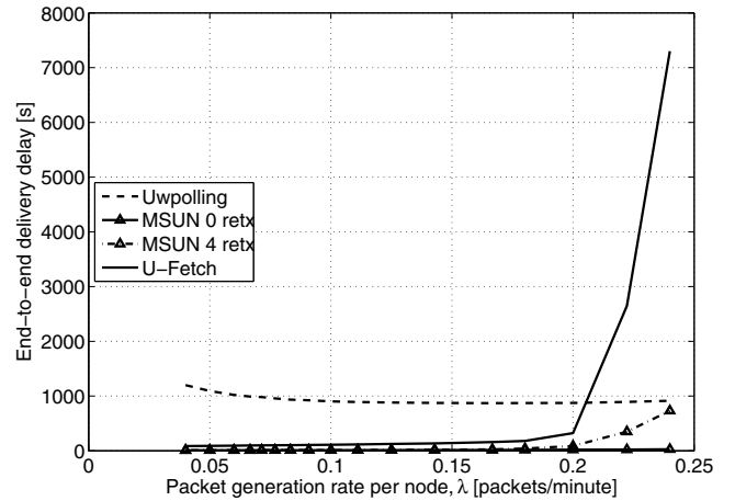
Figure 10. End-to-end delivery delay as a function of the packet generation rate \lambda , in packets per minute per node.
