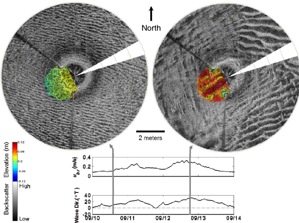
Fig. 4. Composite images of fan sonar backscatter (grayscale images) and azimuth sonar topography (inset colored contour maps) made about two day apart in 12-m water depth about 2 km south of Martha’s Vineyard, MA. Wave conditions (orbital velocity and wave direction) are shown in the time-series plot.
