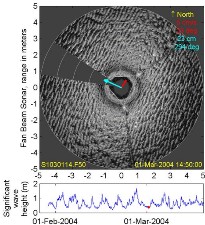
Fig. 2. Fan sonar image with current direction and speed (red) and feature wavelength and direction (aqua, enlarged 5x) overlaid. The bottom frame shows the wave climate during the experiment; the red dot indicates the time of the image.
