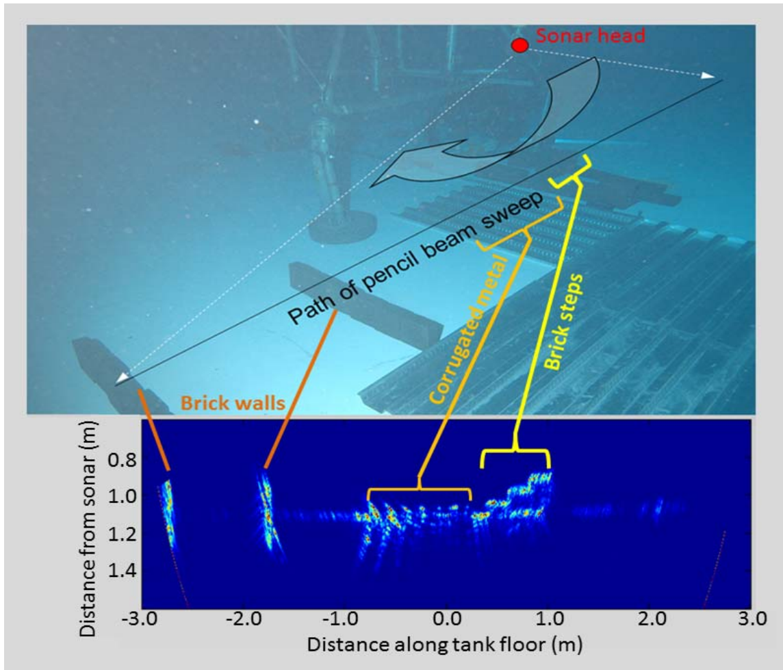
Fig. 3. The top section shows a photograph of the profiling head and the targets used in tests 2-5 with corresponding data from the profiling sonar corrected for -2.4 degree head tilt shown below. Features in the sonar image are connected to corresponding targets in the photograph by colored lines.
