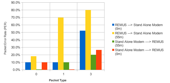
Figure 7. Packet Error Rate vs Packet Type based on experiments between REMUS 100 AUV and a stand-alone WHOI acoustic Micromodem in Loch Earn. Experiments were conducted with the AUV and stand-alone modem next to each other (0m range), and at 55m distant.
