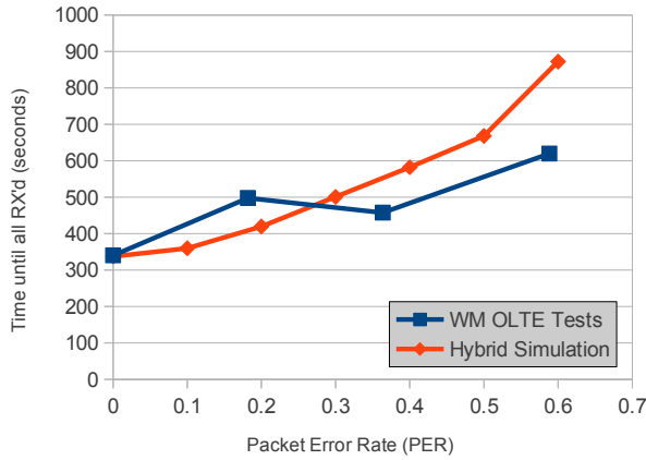
Figure 8. Time to successful reception of all transmitted WM updates, simulation compared to real-world performance. Simulation results were produced using GNU Octave software, while the real-world results were produced in Loch Earn using two stand-alone acoustic Micromodems
