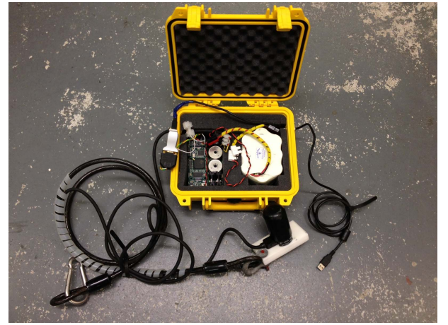
Figure 5. Yellow box (YB) stand-alone modem
