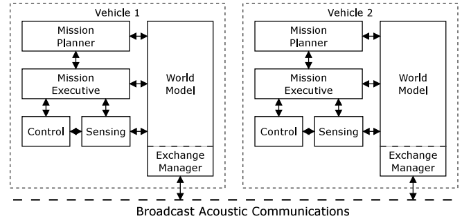
Figure 3. Distributed world model architecture. Figure taken from [1].
