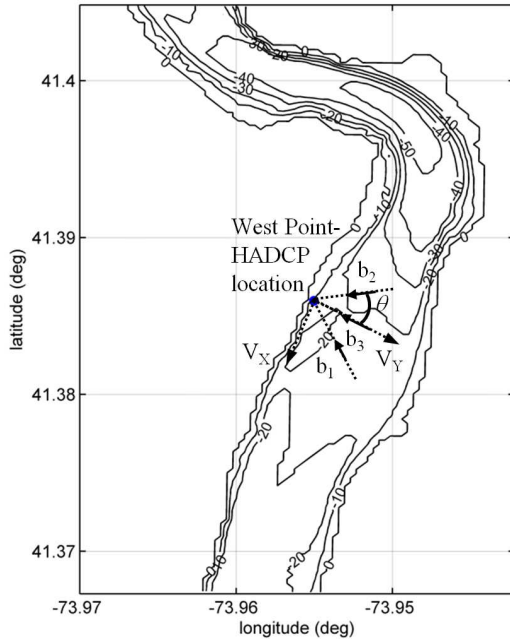
Fig. 1. A reach of the Hudson River around a three-beam HADCP at West Point. Depth contour interval is 10 m
