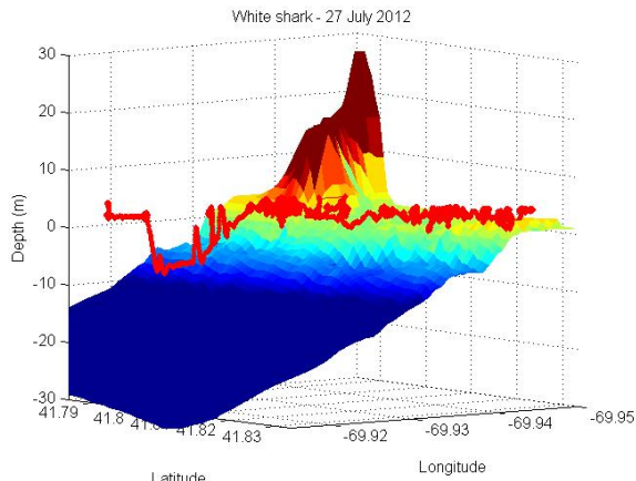
Figure 9. Three-dimensional plot of shark track superimposed on GEOSAT bathymetry set.
