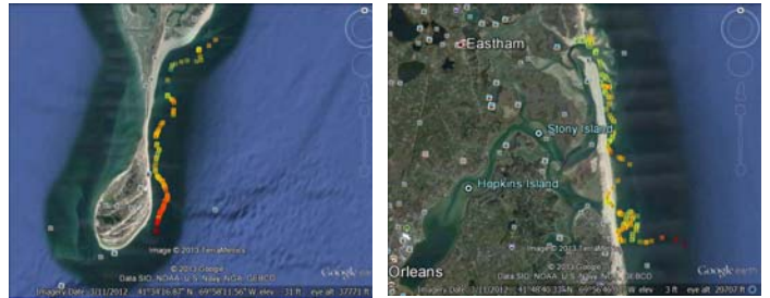
Figure 4. Sample tracks of two white sharks swimming off Monomoy (left) and Orleans (right).
