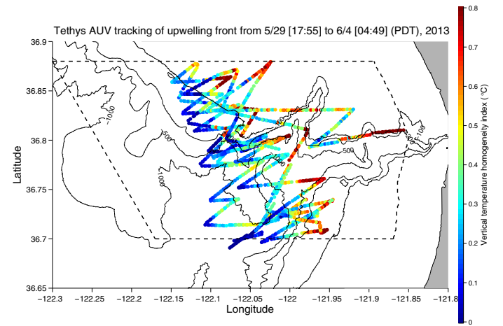
Fig. 5. From 29 May to 4 June 2013, the Tethys AUV autonomously detected and tracked the upwelling front in Monterey Bay. Color on the AUV's track denotes the value of \Delta Temp_{vert} (small in the upwelling water column and large in the stratified water column). The bounds of the AUV's "operational zone" are marked by the dashed lines.
