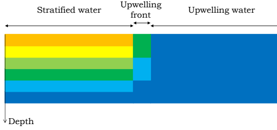
Fig. 1. Illustration of different vertical temperature structures in stratified and upwelling water columns, and in the narrow front between them. Temperature from high to low is represented by color ranging from orange to blue (i.e., the temperature decreases with depth).
