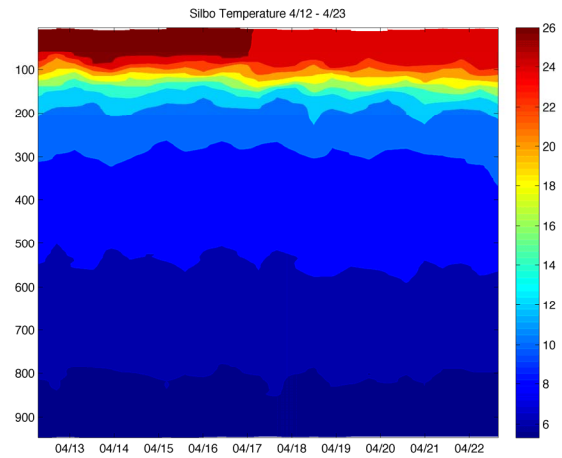
Figure 5b: The temperature dataset from Silbo, used for the case study of 4/12/13-4/23/13.
