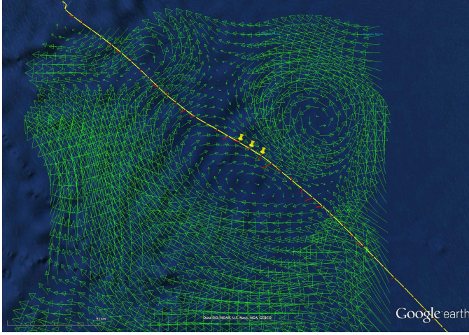
Figure 11a: MyOcean surface current projections and surface currents reported by RU29 for 5/06/2013.
