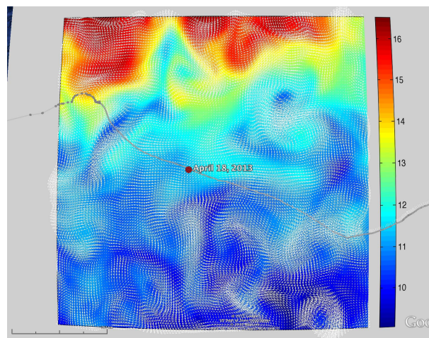
Figure 8b: MyOcean 200m temperature and currents on April 18 th , 2013. The Gliders position is marked by a red dot.
