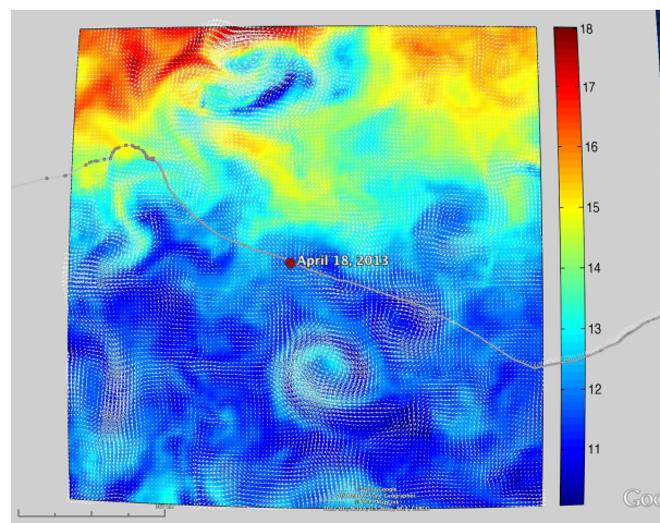
Figure 8a: RTOFS 200m temperature and currents on April 18 th , 2013. The glider position is marked by the red dot.
