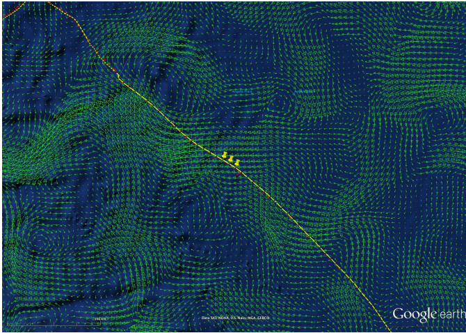
Figure 11b: RTOFS surface current projections and surface currents reported by RU29 for 5/06/2013.
