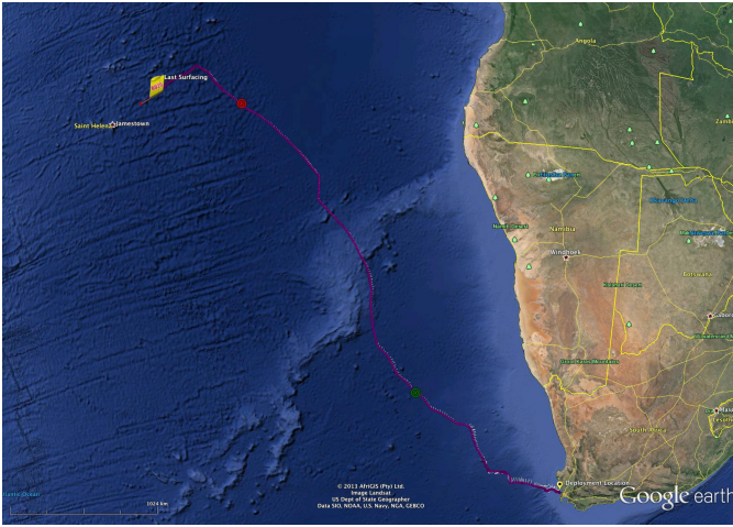
Figure 6a: The portion of RU29's track that was used for comparison to the models, beginning at the green dot and ending at the red dot. This track represents a south to north section along the eastern side of the South Atlantic Gyre.
