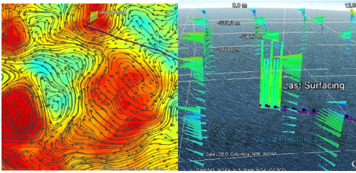
Figure 4: Example of the path planning tools that can be made using data from the ocean forecasting models RTOFS (left) and MyOcean (right).
