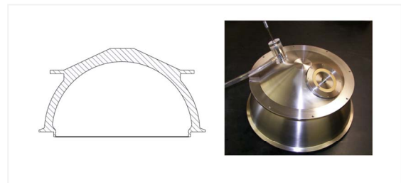
Fig.10 The Nereus main housing end cap with vacuum port sealing assembly
