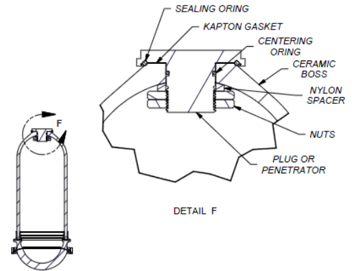
Fig.9 Ceramic boss with floating penetration
