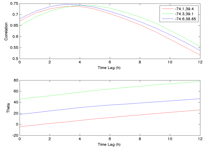
Fig. 2: Time-lag dependent complex correlation magnitude (top) and angle offset between highest correlated components of wind and surface current (bottom) for three points in regions of high correlation (red: northernmost, green: central, blue: southernmost). The correlation peaks at a time lag of around three hours, and offset angle steadily increases with increasing time lag.
