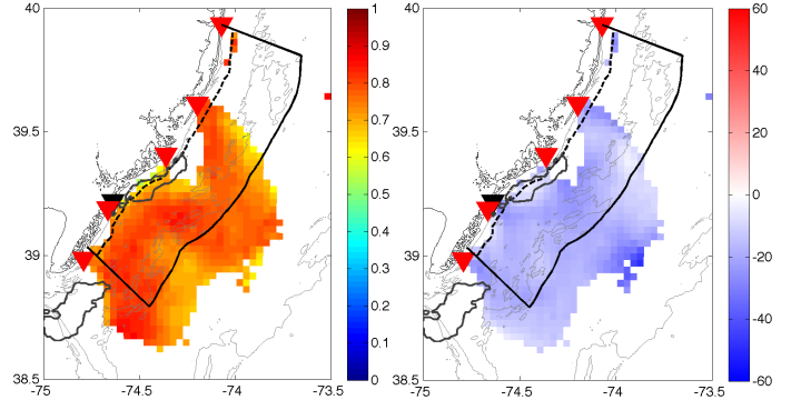
Fig. 6: Magnitude of complex correlation (left) and angle offset (right) between the CODAR-predicted surface wind and RUWRF modeled 10m wind, for the upwelling case. Black triangle: location of the Ocean City WeatherFlow site; Red triangles: 13 MHz CODAR sites; Black solid line: study area; Dashed line: boundary between federal and state waters; Gray solid contour: 22^\circ\text{C} isotherm of SST, showing coastal upwelling.
