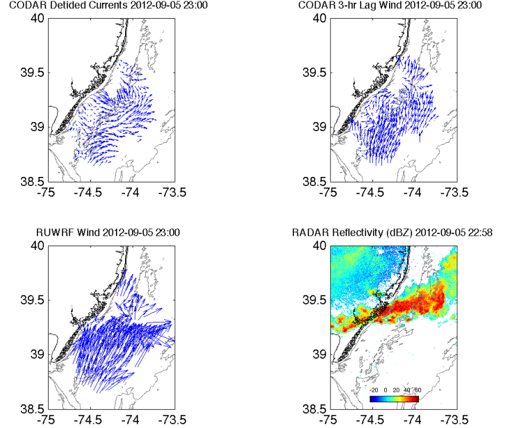
Fig. 8: Detided surface currents on 5 Sep 2012 23:00 GMT (top left), wind predicted for 23:00 GMT based on the currents 3 hrs earlier (top right), RU-WRF model 10m wind at 23:00 (bottom left), and weather radar reflectivity depicting a line of strong thunderstorms at 22:58 GMT (bottom right).
