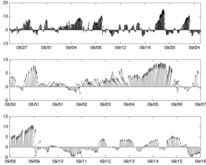
Fig. 1: Hourly 75-minute averaged wind measurements at the Ocean City WeatherFlow site for the time period used to train the surface current-based wind model. Top panel shows winds for the entire time period, middle panel shows the early September 2012 sea breeze case, and the bottom panel shows the mid-September 2012 sea breeze case. Tick marks are at 00:00 GMT for day noted.
