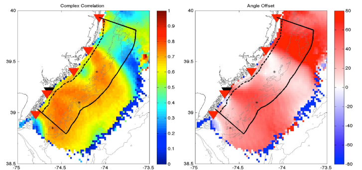
Fig. 3: Magnitude of complex correlation and angle offset between the highest correlated components of the wind and surface currents with a three-hour lag. Black triangle: location of the Ocean City WeatherFlow site, red triangles: 13 MHz CODAR sites, solid line: study area offshore wind (extending 20 nm offshore), dashed line: boundary between federal and state waters (3 nm offshore), asterisks: test locations for time lags shown in Fig. 2.
