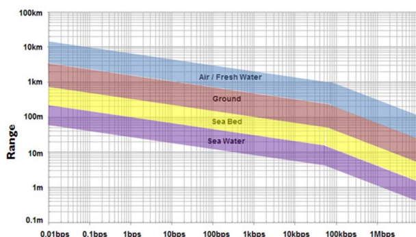
FIGURE 8: Seatooth®, range vs bandwidth
