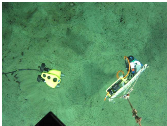
FIGURE 7: A Mini ROV interrogating and wirelessly harvesting data from a subsea sensor
