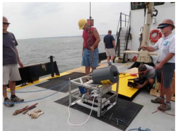
FIGURE 5: The second modem can be seen here built into the seabed frame with the water quality sensor.
