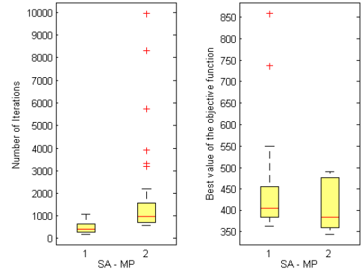
Fig. 7. Comparison of the optimization algorithms with the time-dependent policy representation over 50 experiments.
