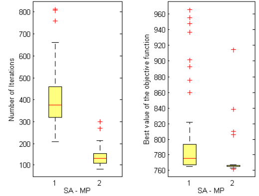
Fig. 4. Comparing the optimization algorithms with constant policies values over 50 experiments.
