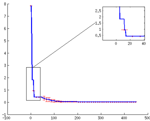
Fig. 13. Computational cost of the learning method to find the (global) optimum solution.
