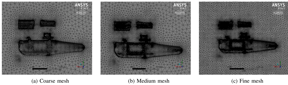
Fig. 8: Grid dependence meshing resolutions shown on the axis of symmetry
