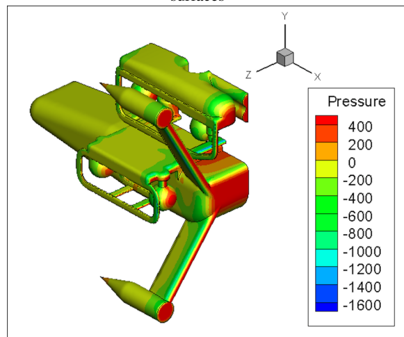
Fig. 9: CFD simulation results for a head-on current of 1 m/s on the Millennium Falcon and AMP
