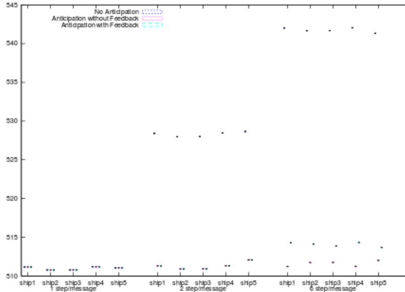
Fig. 12. Individual average of the meeting point results obtained using fuzzy logic when the TS is using 0.8 of its correct speed.
