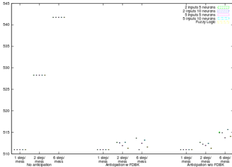
Fig. 8. Global average of the meeting point results for the AUVs obtained with all anticipation models when the TS is traveling at 0.8 of its correct speed.
