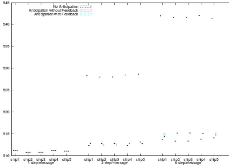
Fig. 10. Average and quartile results for the meeting point by AUV, when using a neural network with 10 inputs and 5 neurons in the hidden layer when the TS is using 0.8 of its correct speed. All AUVs have similar errors, showing that they remain together. Errors are much larger when there is no anticipation and a messages are infrequent.
