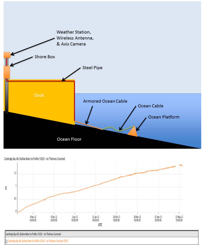
Fig.6. A schematic diagram of the nearshore cabled ocean observatory (upper panel) at Cambridge Bay, NWT Canada [11] which was installed in September 2012. The lower panel displays the real-time ice thickness data obtained from a Shallow Water IPS5 instrument from October 2102 (ice formation) through to May2013.
