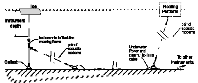
Fig.7. A schematic diagram of a remote real-time deep-water cabled observatory system [16].
