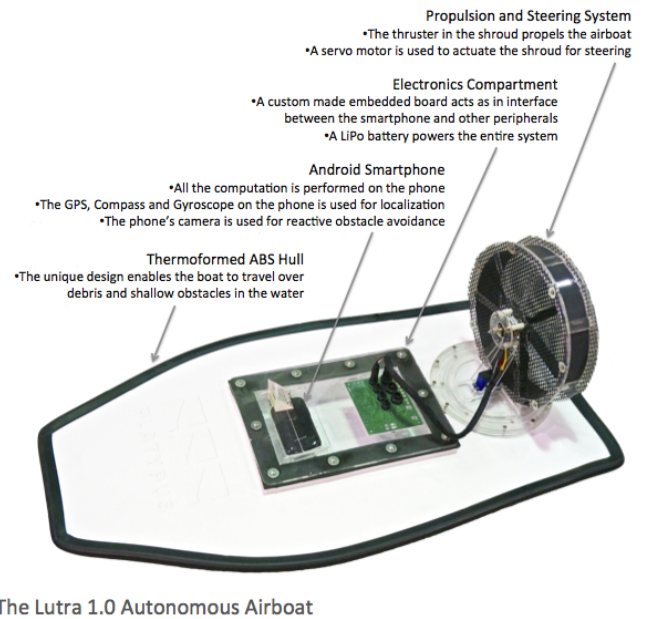
Fig. 2: A Complete Lutra 1.0 Series Autonomous Airboat
