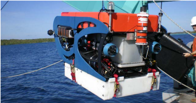
Figure 8. WHOI Hybrid High Definition 3D Cinematography ROV
