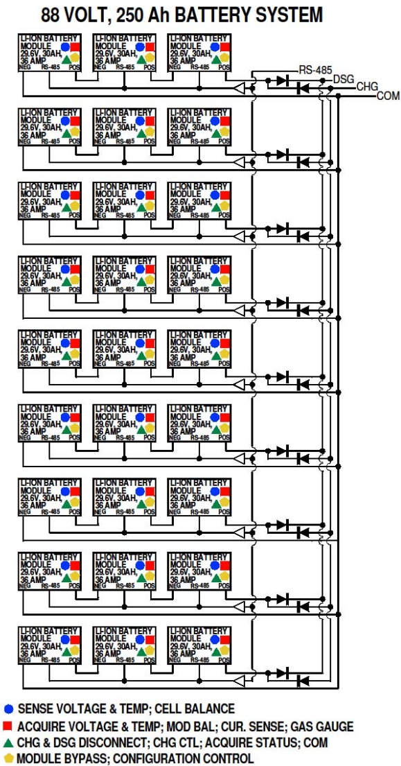
Figure 6. 3S9P Autonomous Battery Modules
