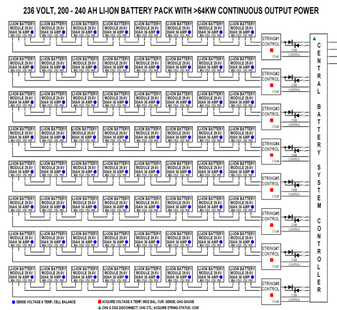
Figure 2. Example Centralized Architecture Lithium-Ion Battery System
