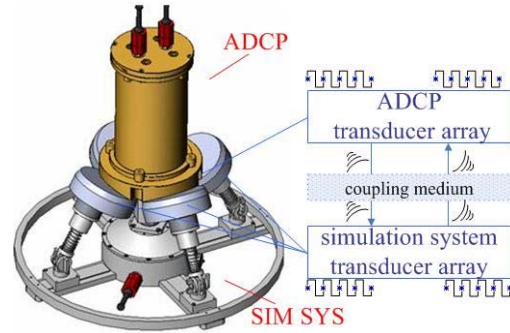
Figure 1 Schematic diagram of the simulation system dock structure
