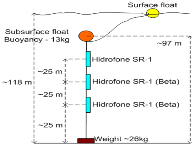
Fig. 5. Mooring with 3 SR-1 hydrophones.
