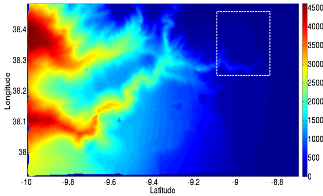
Fig. 1. Bathymetry of the Sesimbra region (depth in meters), showing the area of operation (white box)
