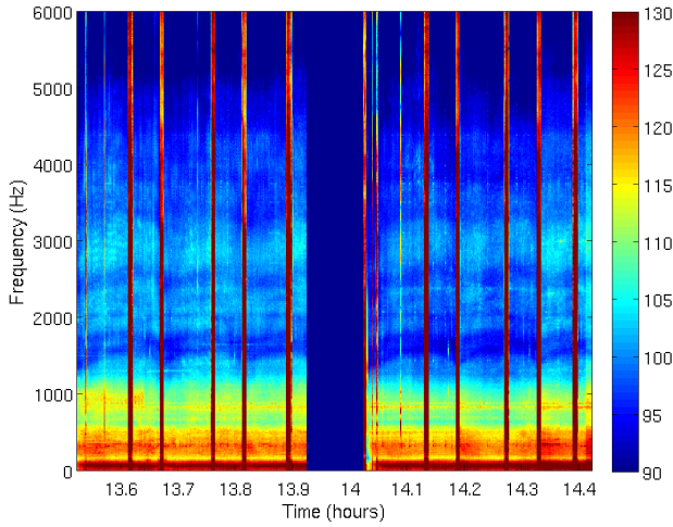
Fig. 14. Noise registered by SR-1 carried by the glider (zoom).
