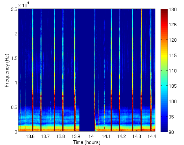
Fig. 13. Noise registered by SR-1 carried by the glider.
