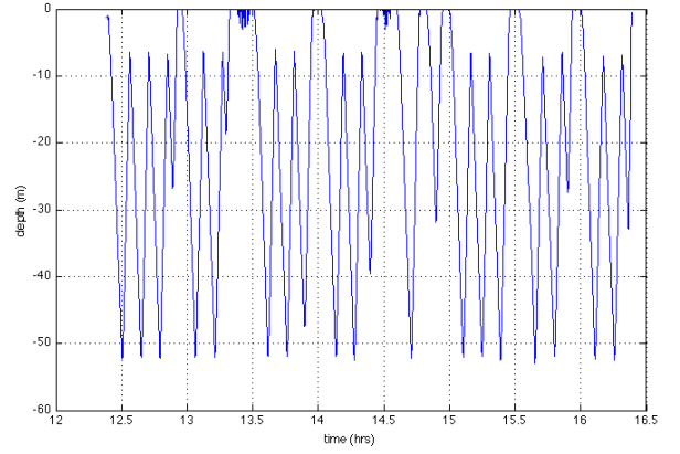
Fig. 12. Glider depth profiles (day 3 afternoon).
