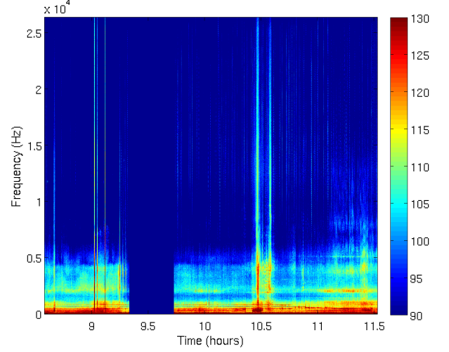
Fig. 9. Noise registered by SR-1 towed by FAST.
