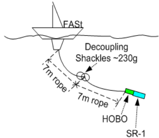
Fig. 7. FAST towing a SR-1 hydrophone.
