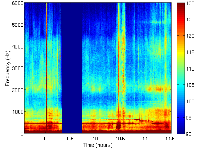
Fig. 10. Noise registered by SR-1 towed by FAST (zoom).
