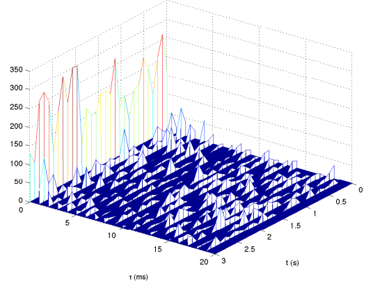
Fig. 2. Channel impulse response for 30 consecutive chirps at the first receive element in the first environment, these estimates have been computed from the data recorded on July 2nd, 2011 at 3:24.
