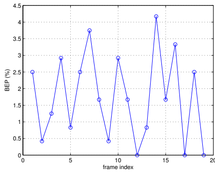
Fig. 3. The uncoded error probability of the chirp parameters at rate equals to 107bps, the table shows the uncoded BEP resulted from using majority voting combining technique.
