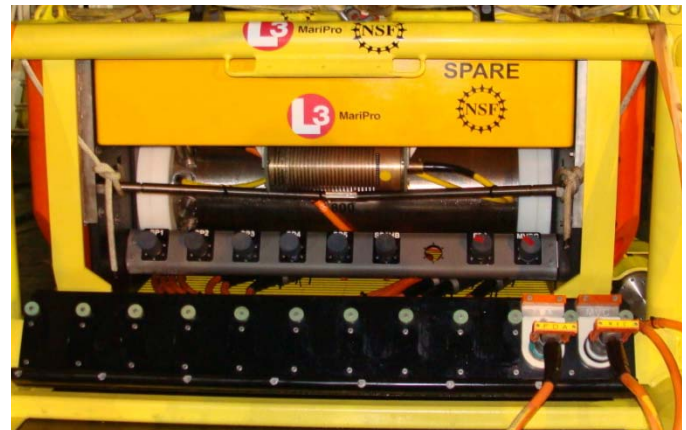
Fig. 4. SIA Wet Mate Connectors
