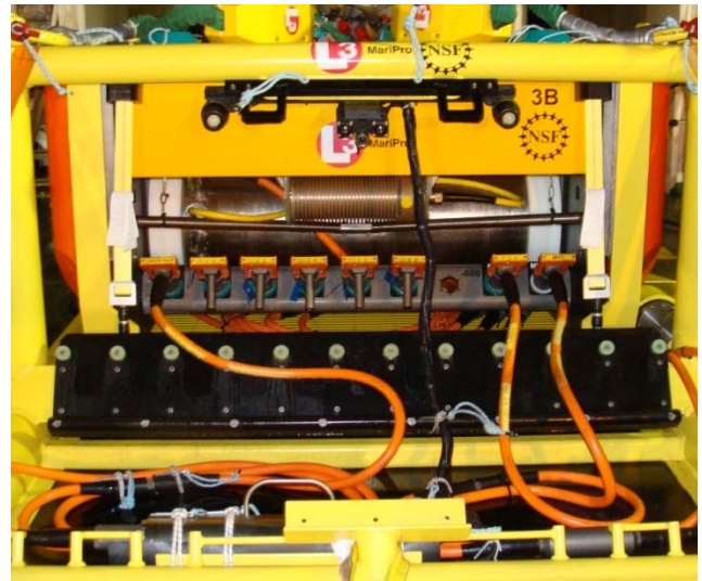
Fig. 7. CSH with Camera System
