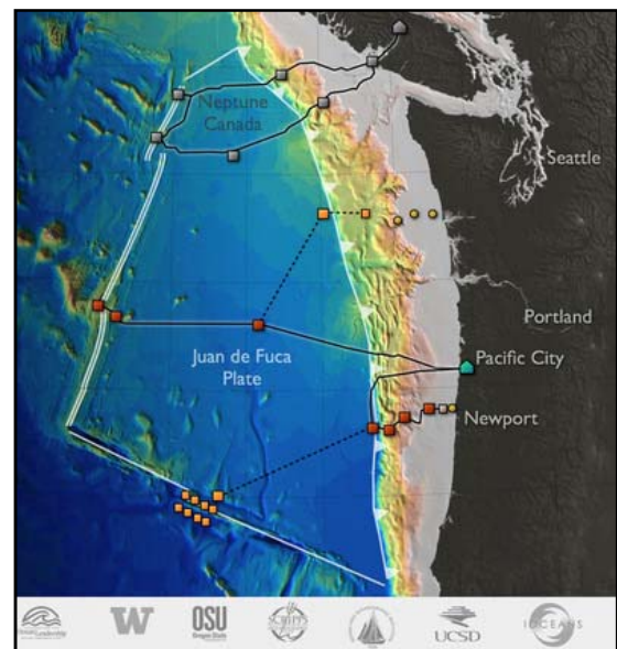
Fig. 1. RSN and NEPTUNE Canada Systems (figure courtesy of UW)
