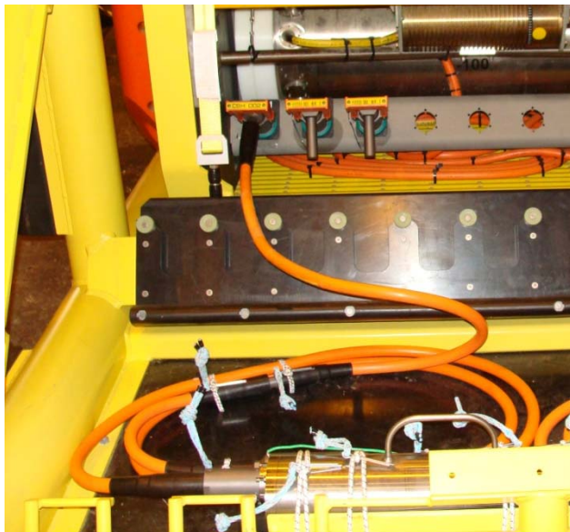
Fig. 6. CSH Mounted on Node and Connected to SP1
