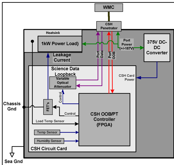
Fig. 5. CSH Simple Block Diagram
