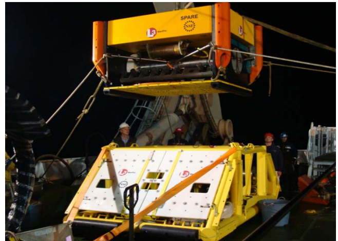
Fig. 3. SIA Being Installed into a BIA
