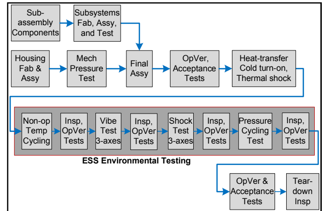
Fig. 9. Typical Qualification Test Flow
