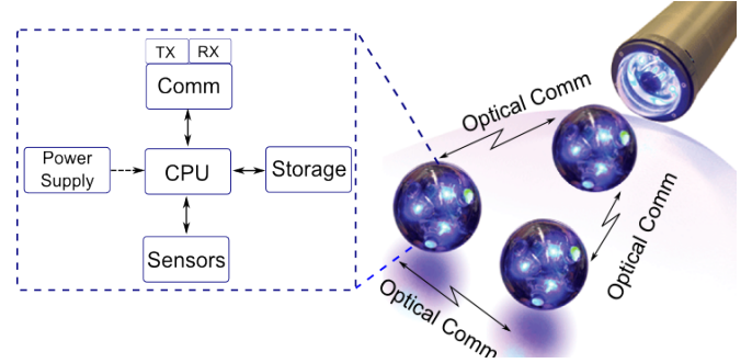
Figure 1. The Sensorbot optical communications network and subsystems diagram.
