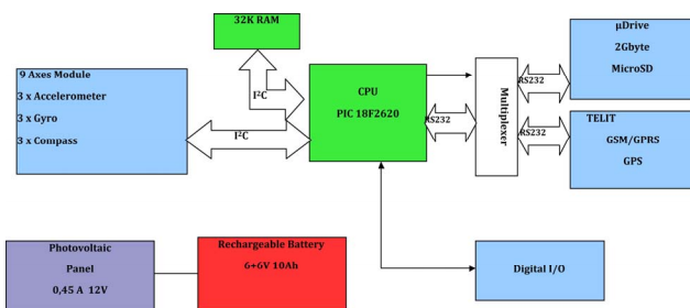
Fig. 3. Geo-referenced system
