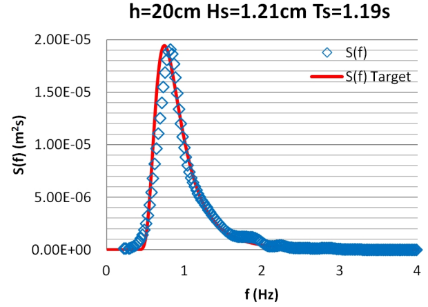
Fig. 7. Comparison of target and incident wave spectra
