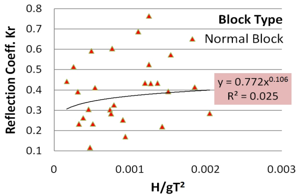
Fig. 11. Reflection ratios for normal block placement and reverse direction.
