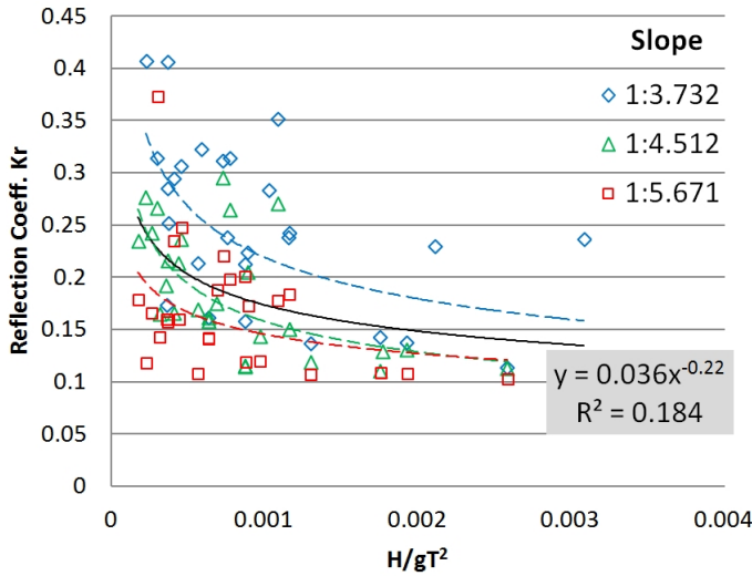
Fig. 16. Reflection ratios for eco block placement with respect to slopes.
