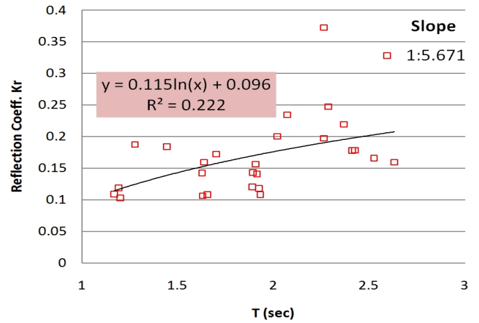
Fig. 13. Reflection ratios versus wave period for eco block placement. (slope 1:5.671)
