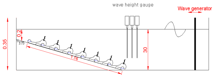
Fig. 5. Wave flume and experimental setup.
