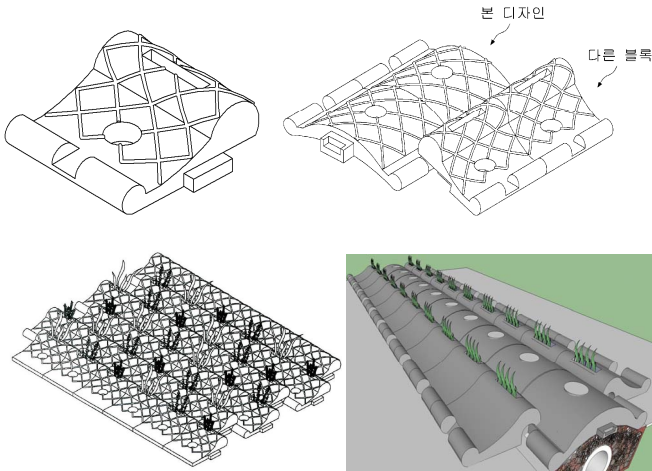
Fig. 17. Schematic view of developed bio blocks.
