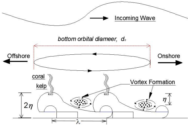
Fig. 3. Schematic diagram for water motion and eco blocks.
