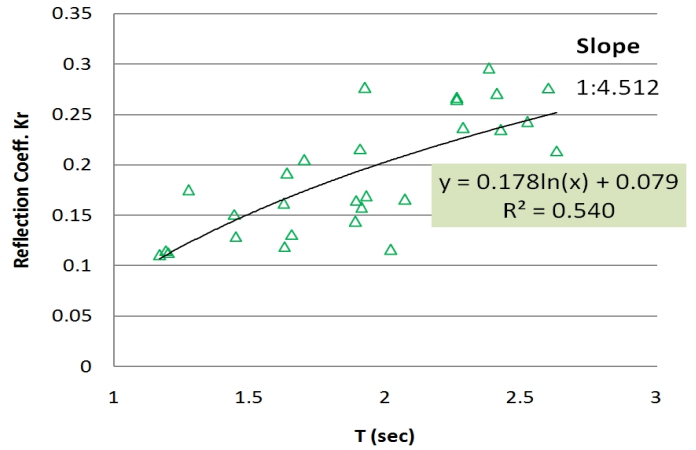
Fig. 14. Reflection ratios versus wave period for eco block placement. (slope 1:4.512)
