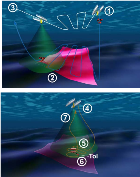
Fig. 1. The TRIDENT strategy. ( Top ) The initial stage focused in the survey task: (1) I-AUV deployed; (2) Coordinated Survey; (3) I-AUV surfaced. ( Bottom ) The final stage in charge of the intervention mission: (4) ASC dynamic position; (5) I-AUV looking for Target of Interest (ToI); (6) Grasping; (7) I-AUV docks to the ASC.
