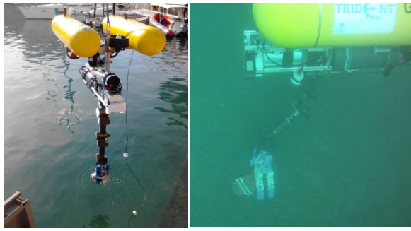
Fig. 6. Final intervention experiments in Söller: (Left) I-AUV deployment. (Right) Successful intervention.
