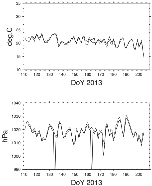
Fig. 5. Surface temperature (degree C) and air pressure (hPa), compared with NCEP/Reanalysis values (dashed line).
