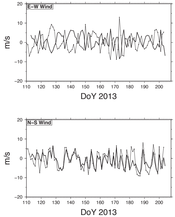
Fig. 4. The EW and NS components of the wind velocity measured by the buoy anemometer (solid), compared with the NCEP/Reanalysis wind data (dashed). Note that the EW component is out of phase with the NCEP data, due to an error in the datalogger program. This problem has been fixed for the second buoy.
