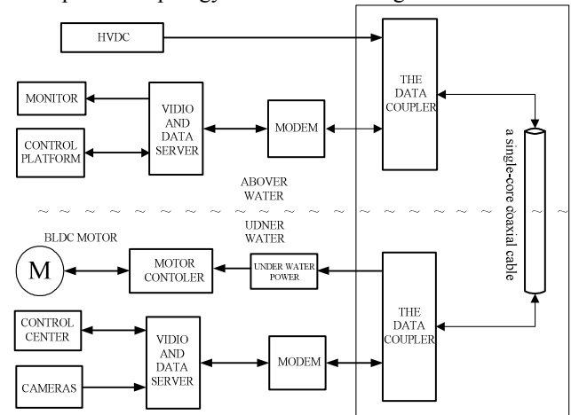
Fig.1 Block diagram of a hybrid transmission system
