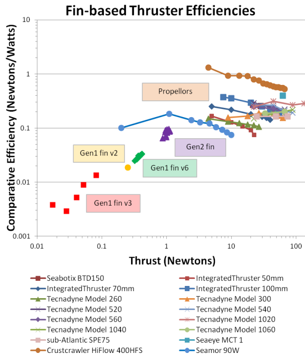
Fig. 12. A comparison between pectoral fin (bottom left data points) and traditional thruster (top right data curves) efficiencies.
