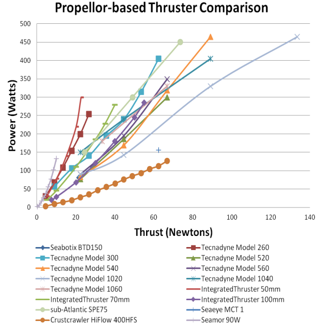
Fig. 1. Forward Thrust vs. Power consumption curves of several off-the-shelf propeller based thrusters.
