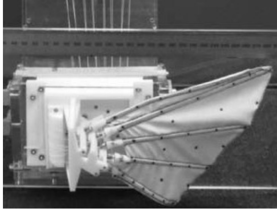
Fig. 7. The Tangorra fin, modeled from a sunfish pectoral (Gottlieb, 2010).
