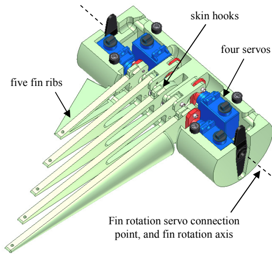
Fig. 6. The internals of the Gen2 fin. Dual fin rotation servos not shown.
