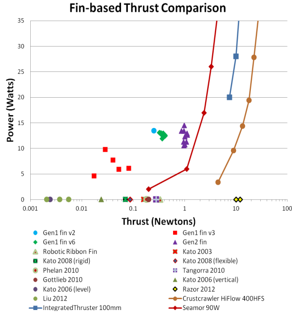
Fig. 10. Power and thrust of bio-mimetic pectoral fins compared with traditional thrusters.
