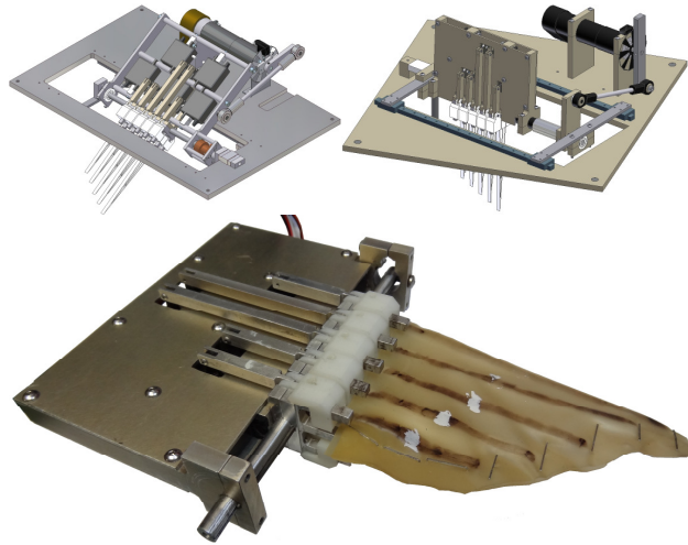
Fig. 3. The Gen1 fins: v2 (top left), v3 (top right), v3 without fin rotation motor (bottom).
