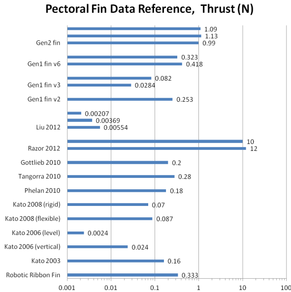
Fig. 11. Reference chart of pectoral fin thrust data.
