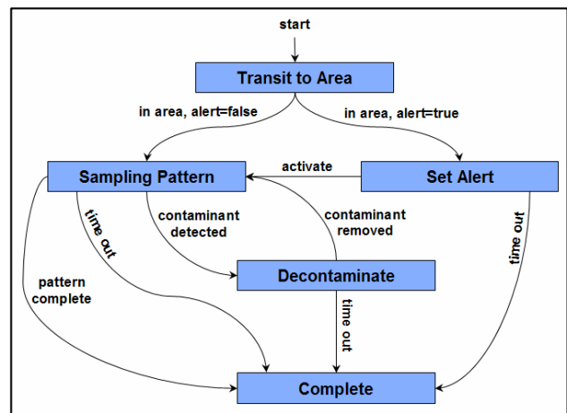
Figure 9. Strategic goal task algorithm for Decontaminate [17]. Completion status can only result in success or failure.
