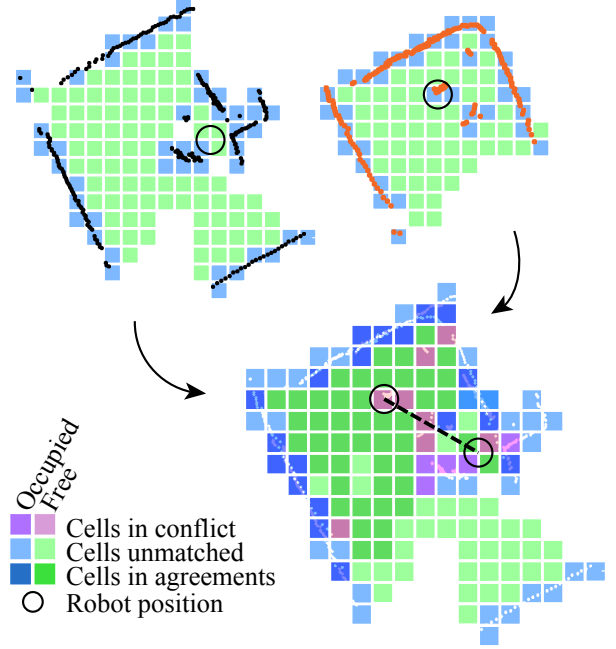
Figure 4: Step 7 of the LatticeMap algorithm: Scan matches are raytraced to produce occupancy grids, then overlayed. Cells in agreement add to the matchings score.
