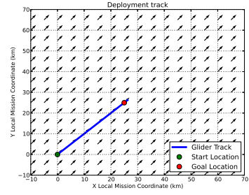
(c) Current correction enabled with the new heading correction algorithm.
