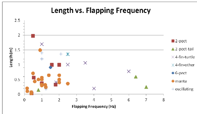
Fig. 5 A comparison of UUV length vs. flapping frequency. No allometric relationship found.
