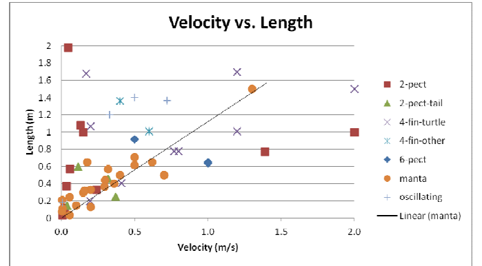
Fig. 3 A comparison of UUV velocity vs. length.
