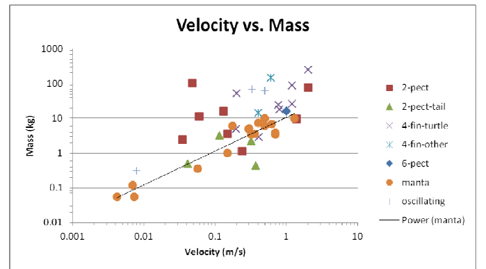
Fig. 4 A comparison of UUV velocity vs. mass.
