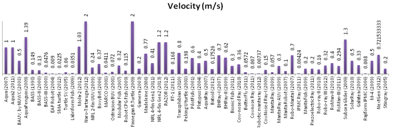
Fig. 8 A reference of UUV velocity data.
