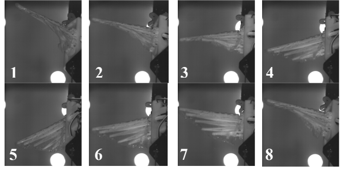
Fig. 1. Example fin surface curvature for an entire flap cycle.
