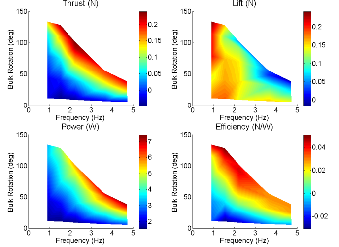
Fig. 6. Passive gait results across all frequency and bulk amplitudes. max thrust is 0.24 N at \theta=102^\circ , f=2.2 Hz, power = 5.8 W
