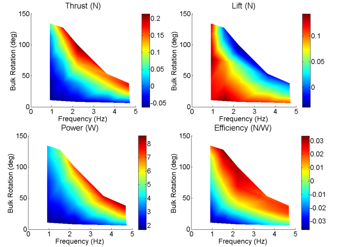
Fig. 7. Rigid gait results across all frequency and bulk amplitudes. max thrust is 0.21 N at \theta=100^\circ , f=2.2 Hz, power = 7.2 W
