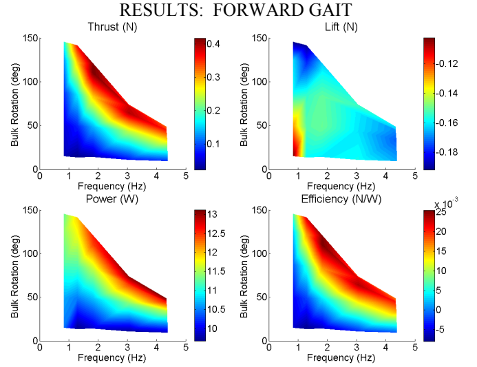
Fig. 3. Forward gait results across all frequency and bulk amplitudes. max thrust is 0.42 N at \Theta=111^\circ , f=1.8 Hz, power=12.4 W
