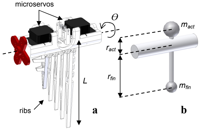
Fig. 9 a) Pectoral fin design, and its b) point mass representation.
