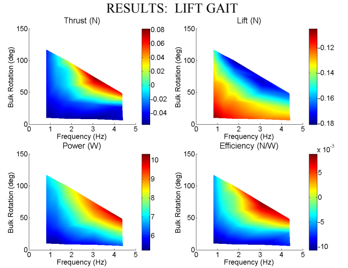
Fig. 4. Lift gait results across all frequency and bulk amplitudes. Max lift is -0.18 N at \Theta=100^\circ , f=1.8 Hz, power=8.1 W
