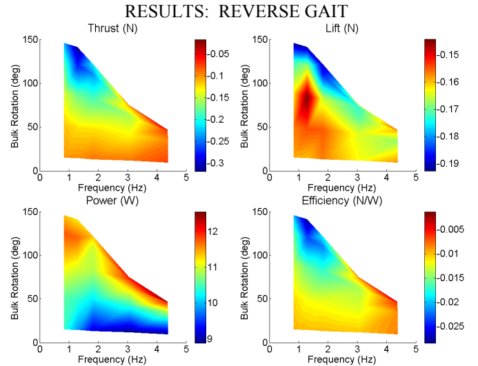
Fig. 5. Reverse gait results across all frequency and bulk amplitudes. max reverse thrust is -0.32 N at \Theta=141^\circ , f=1.3 Hz, power=11.2 W
