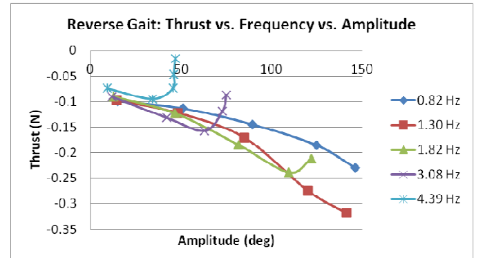
Fig. 11. Thrust output for reverse gait.
