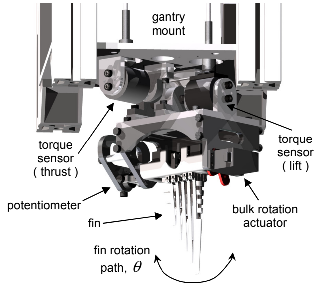
Fig. 2. Experimental force measurement device with fin.
