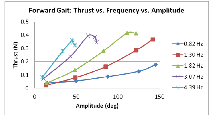
Fig. 10. Thrust output for forward gait
