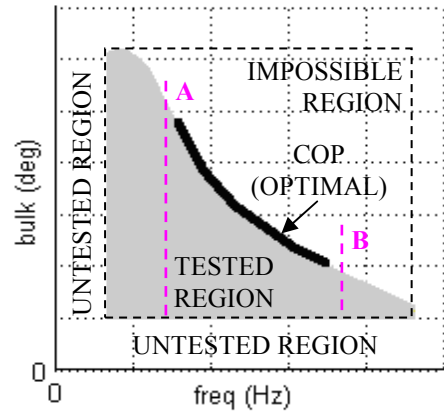
Fig. 8. Guide to Pectoral Fin Brute-Force Testing Results: Untested Region – poor fin performance Impossible Region – fin is incapable of this bulk/freq. combo Tested Region – region where results were obtained Between A and B – desired region for standard fin operation
