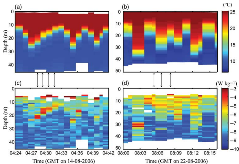
Figure 8. (a and b) Temperature (°C) and (c and d) dissipation rate of turbulent kinetic energy, \epsilon ( \text{W kg}^{-1} ), on a log scale, as measured by the direct microstructure profiler on 14 and 22 August 2006. The measurements were collected at the same time as the broadband acoustic data illustrated in Figure 7. The arrows indicate the profiles plotted in Figure 11 for comparison with the acoustic inferences of \epsilon .
