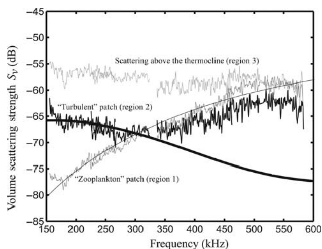
Figure 10. Measured scattering spectra of the regions labelled 1–3 in Figure 7c and d during the passage of a non-linear internal wave on 22 August 2006. The thin solid grey line represents the predicted scattering from elastic-shelled pteropods based on inferred size and abundance from least-squares inversions ( r^2 = 0.98 , p < 0.01 ). The thick solid black line represents the predicted scattering from turbulent microstructure based on inferred values of the dissipation rate of turbulent kinetic energy, \varepsilon ( \text{W kg}^{-1} ) and temperature variance, \chi_T ( \text{m}^2 \text{s}^{-1} ; r^2 = 0.68 , p < 0.01 ).
