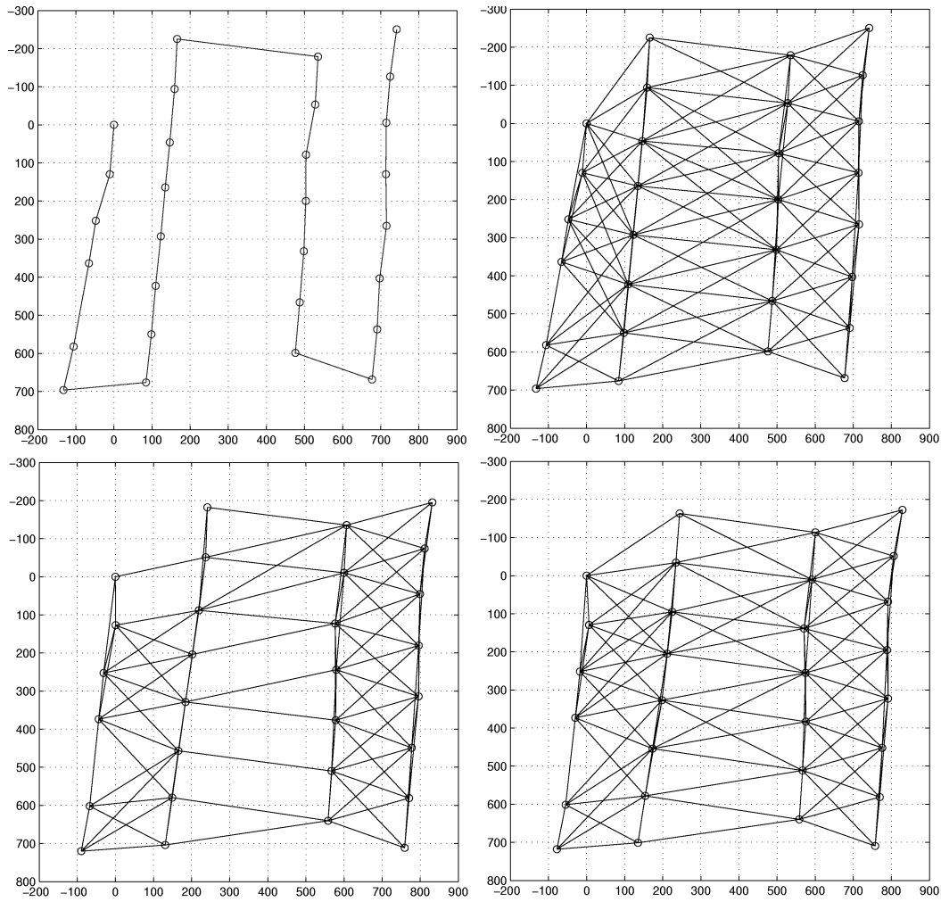
Fig. 13. (Top left) Image layout after initial topology estimate (using only temporal overlap information) and proposed links based on possible overlap given the topology estimate (top right). (Black is for verified links and gray is for proposed ones.) Axes correspond to mosaic coordinates (in pixels). Image layout after second (bottom left) and final (bottom right) topology refinements. (Only verified links are shown.)
