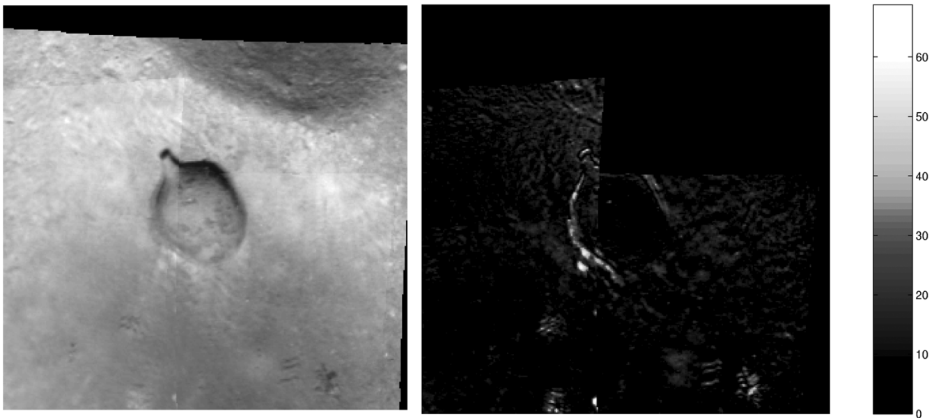
Fig. 20. Detail of top-right corner of the radiometrically corrected mosaic in Fig. 18. Average (left) and standard deviation (right) of overlapping source samples. Notice that most of the variability due to lighting differences between overlapping images has been removed (compare to Fig. 16).
