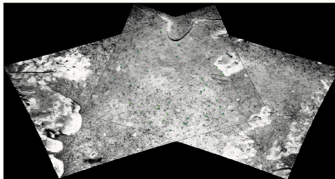
Fig. 12. Mosaic based on matching shown in Fig. 11. Rendered as average of intensities.
