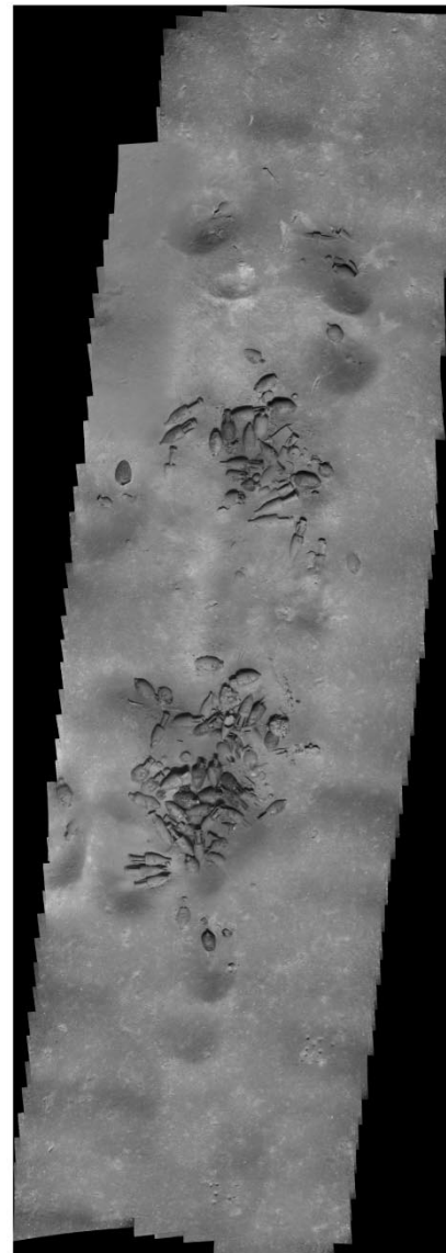
Fig. 33. Multiresolution blended mosaic of the complete Skerki D wreck (233 images) covering an area of approximately 350 m 2 , based on the tessellation of Fig. 32. Images were radiometrically corrected as described in Section IV-3 and corrected for radial distortion using the approach described in Section V.
