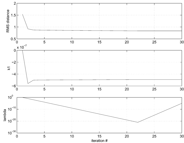
Fig. 24. Evolution of (top) RMS distance of corresponding points on the mosaic, (middle) the radial distortion coefficient, and (bottom) the weighting factor used in the Levenberg–Marquardt algorithm to switch from Newton–Gauss to gradient descent. Note that the radial distortion parameter reduces the RMS distance by more than 50%.
