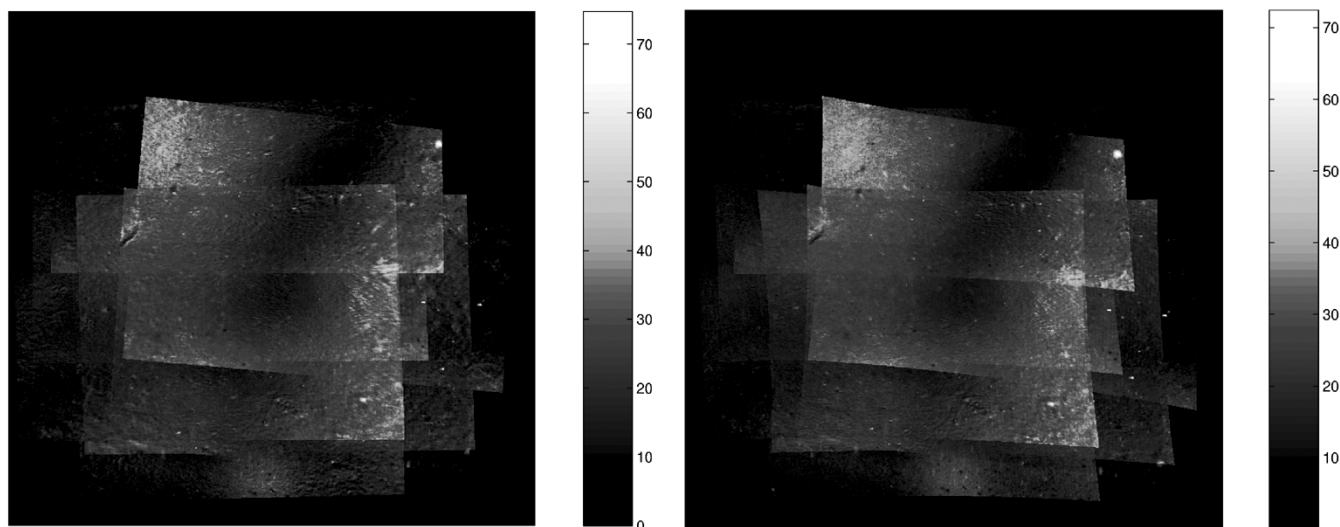
Fig. 28. Standard deviation of source samples at each mosaic sample before and after radial-distortion compensation. Note the reduction of the high-frequency content in the radially compensated mosaic. This indicates improved registration, in particular near image corners.
