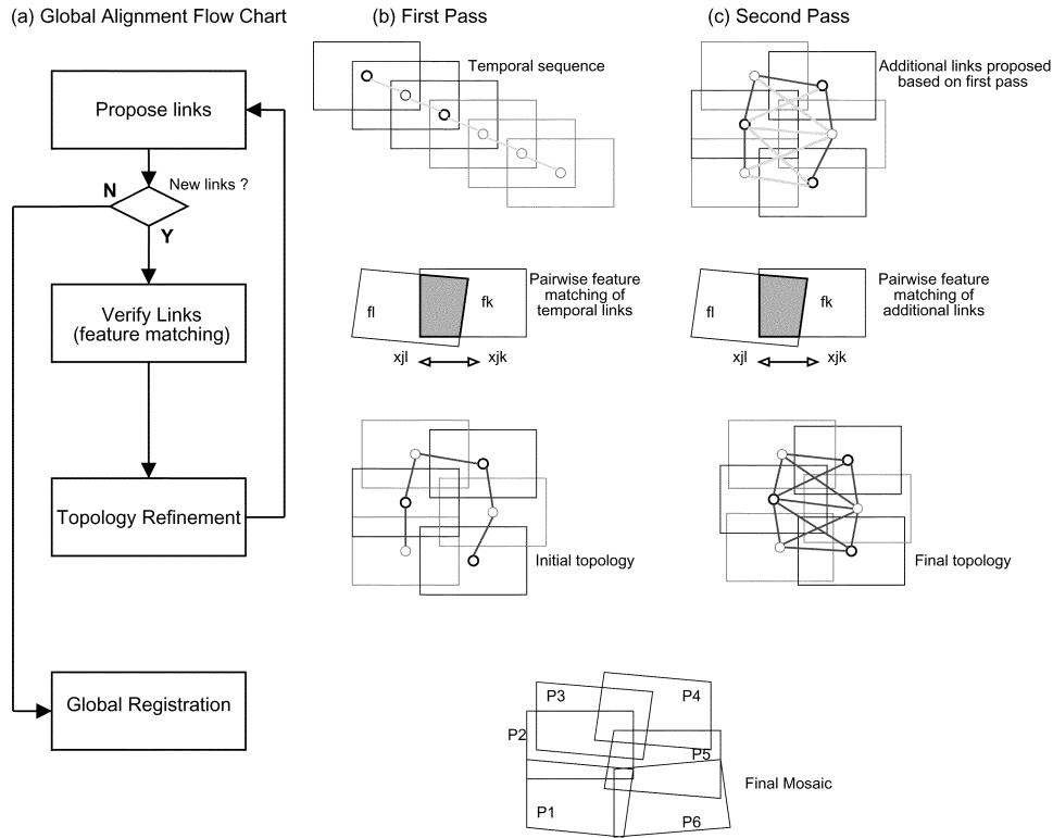
Fig. 4. (a) Flowchart for mosaicing with global alignment through topology estimation. (b) and (c) illustrate the process for a set of six images. Proposed links (based on possible overlap given the current topology estimate) are depicted in light gray, verified links (based on a successful feature matching) in black. Feature matching is represented for the j th feature x_j between images f_l and f_k as x_{jl} \longleftrightarrow x_{jk} .
