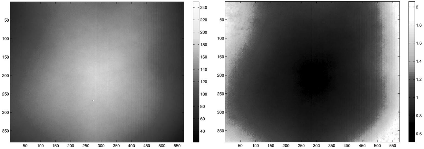
Fig. 17. Average of pixel values over all images of approximately flat sections of the Skerki D wreck (left) and the multiplicative radiometric correction factors (right).
