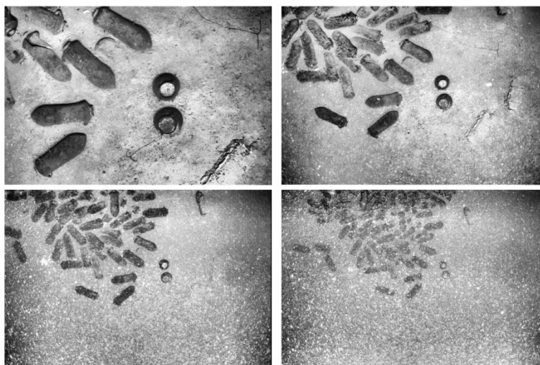
Fig. 2. Set of images taken at different altitudes (from 3.5 to 12.5 m in 3-m increments). Light attenuation and backscatter limit the altitude from which images can be acquired. Covering an area of interest may require several hundreds of images.
