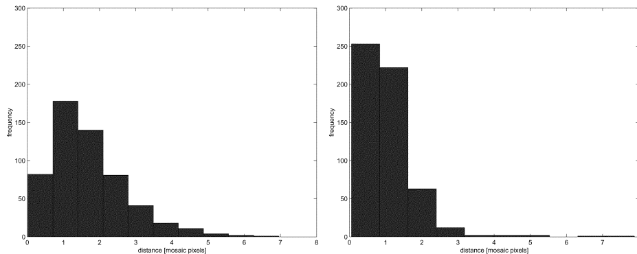
Fig. 25. Distribution of distances between corresponding points on the mosaic, (left) without radial distortion compensation and (right) with distortion compensation.
