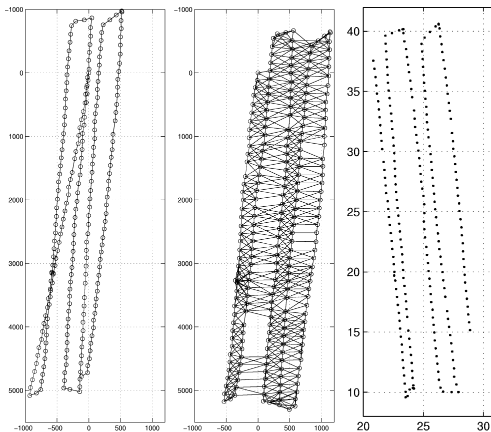
Fig. 29. (left) Initial and (center) final topology for the mosaic of Skerki D wreck site (axes in pixels). The origin for the topology is the center of the first image. Note that the relative position of the first trackline (depicted in gray) shifts dramatically from the initial to the final topology. The resulting mosaic is shown in Fig. 30. The vehicle nav-based position (right), in meters, at the instants the images were taken (with the exception of the last images where nav records are missing). The position was estimated using a 300-kHz-long baseline acoustic net and a Doppler velocity log, with centimeter-level accuracies [64]. The origin for position is the survey origin. The vehicle-navigation data is oriented with north in the +Y direction, whereas the mosaic orientation simply minimizes the overall rotation of the images. The first image of the mosaic corresponds to the westernmost image. The overall shape of the mosaic corresponds to the shape of the survey; notice the relative spacing of the tracklines and instances with larger spacing between consecutive images.
