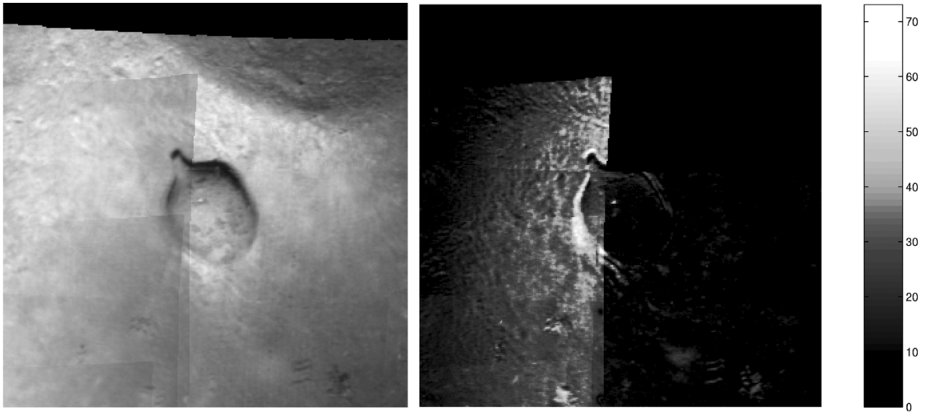
Fig. 16. Detail of top right corner of the mosaic in Fig. 14. Average (left) and standard deviation (right) of overlapping source samples. The misregistration is apparent in the ghosting around the amphora and the blurred terrain in the image of the average. In the standard-deviation image, repeated edge-like structures represent misregistration, while areas with high but approximately uniform variability suggest differences in lighting between the overlapping images.
