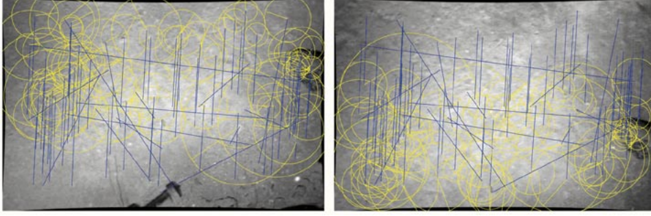
Fig. 6. Matched points according to minimum distance of feature vectors (74 matching pairs out of the 400 feature points in each image). The circles represent the characteristic scale of the feature and the blue lines indicate the interimage motion of the features. Notice that, along with a number of consistent matches (vertical), we also obtain numerous inconsistent matches across the two images.
