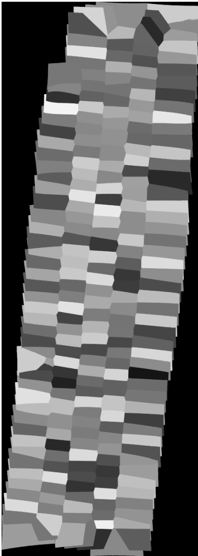
Fig. 32. Tessellation used in the multiresolution blended mosaic of the Skerki D wreck.
