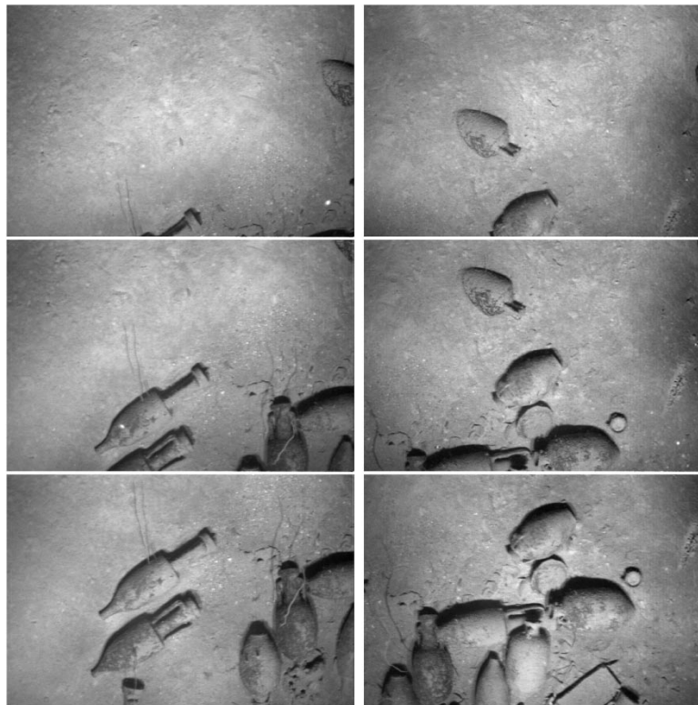
Fig. 3. Sample of the set of 29 images used as a working example to illustrate some of the stages of the mosaicing process. Each column represents a section of adjacent survey tracklines. Images in a column represent a temporal sequence (the vehicle moved down the left column and up the right column with approximately constant heading). Note the low spatial overlap and the failure of the BCC, due to underwater lighting.
