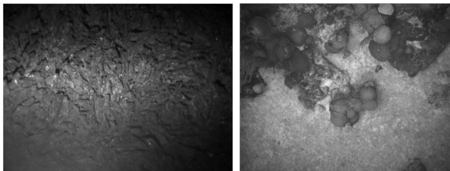
Fig. 1. Sample images from a lava flow and a coral reef survey performed by AUVs. The strong falloff in lighting is typical of energy-limited vehicles.
