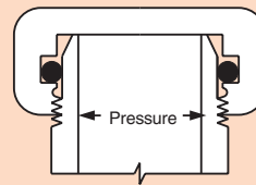
Use the system pressure to close clearance gap.
