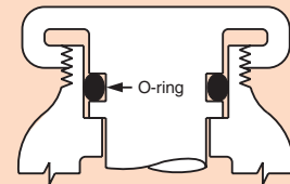
Added wall support on plug seal minimizes breathing. External threads prevent O-ring damage during assembly.
