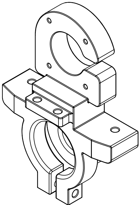
ISOMETRIC VIEW FOR REFERENCE ONLY
