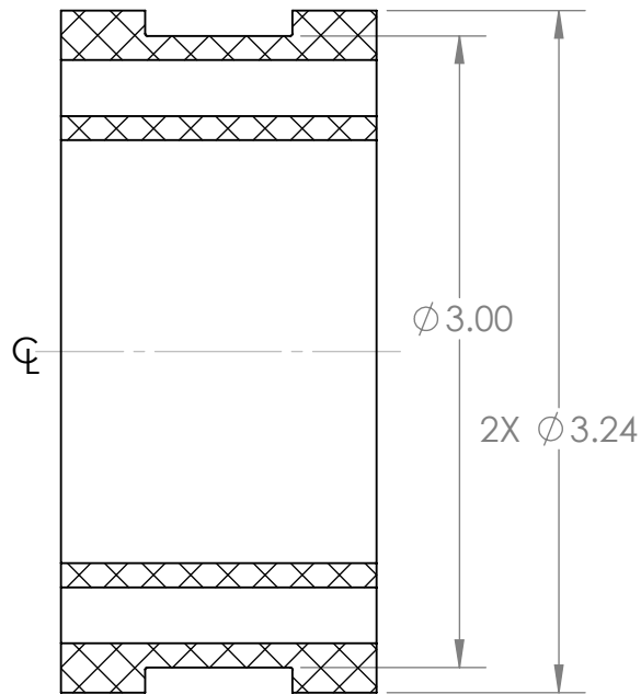
SECTION C-C
