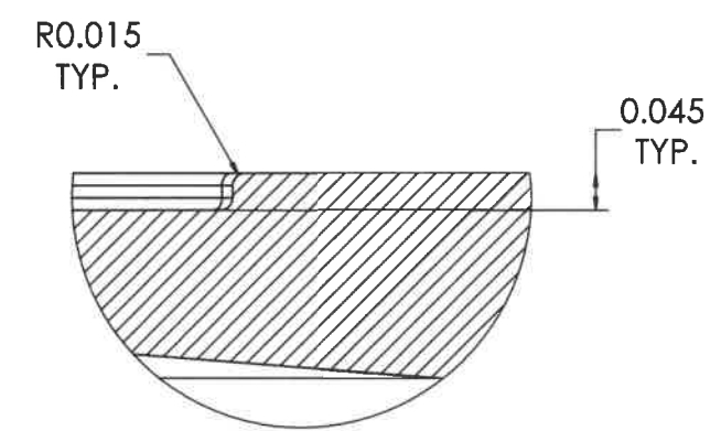
DETAIL A SCALE 8 : 1
