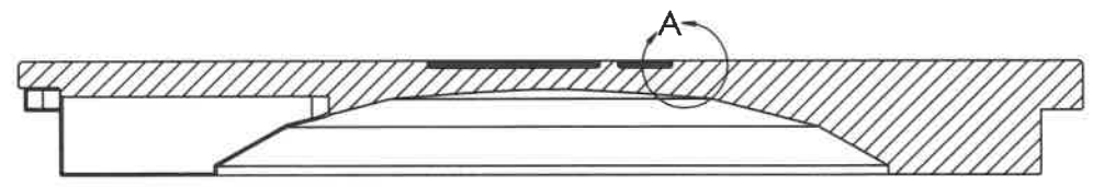
SECTION Y-Y SCALE 1.5 : 1
