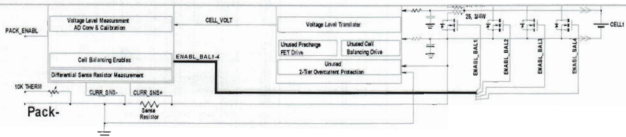
Figure 4 Discharge Module Balancing Circuit
