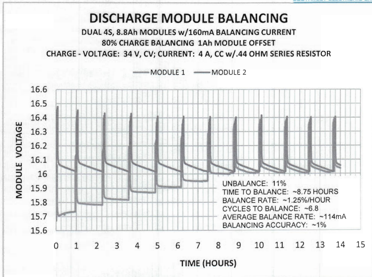
Figure 5 – Discharge Module Balancing Example
