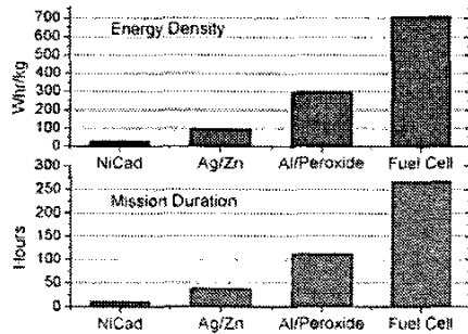
Figure 3. Comparative energy densities.
