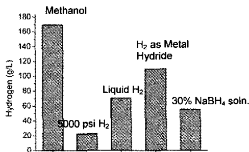
Figure 2. Comparative hydrogen volumetric storage capacities.
