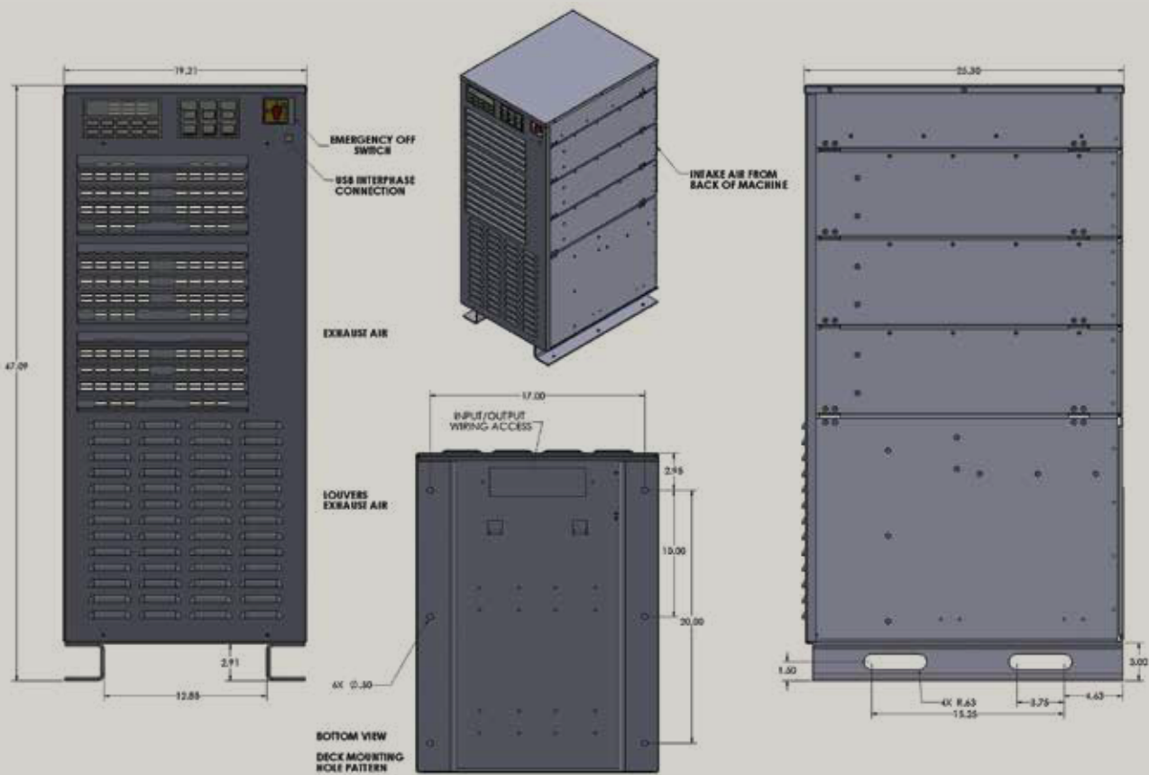
Cabinet Style "AC36Q/AC45Q"
