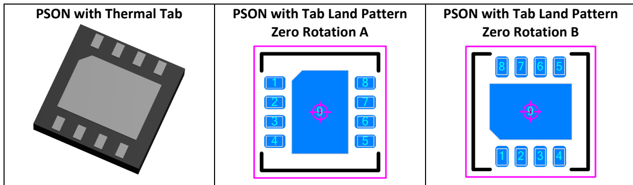
Pull-back Small Outline No-lead (PSON) with Thermal Tab
