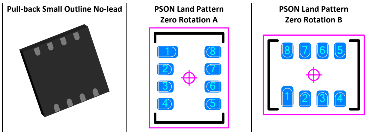
Pull-back Small Outline No-lead (PSON)
