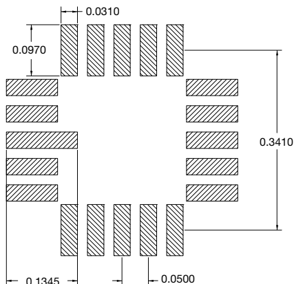
20 Pin LCC
