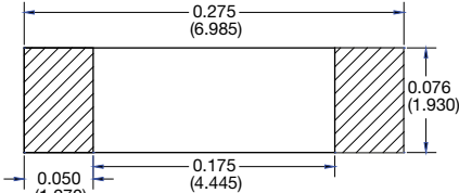
2208 Land Pattern
