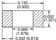
1005 Land Pattern
