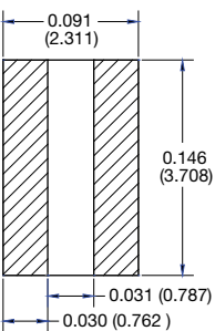
0612 Land Pattern
